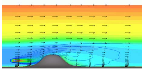
(a) Smoke source height=0.5h
