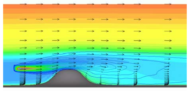
(b) Smoke source height=1.0h
