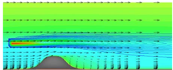
(c)Smoke source height=2.0h
