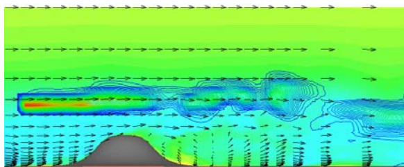
(c)Smoke source height=2.0h
