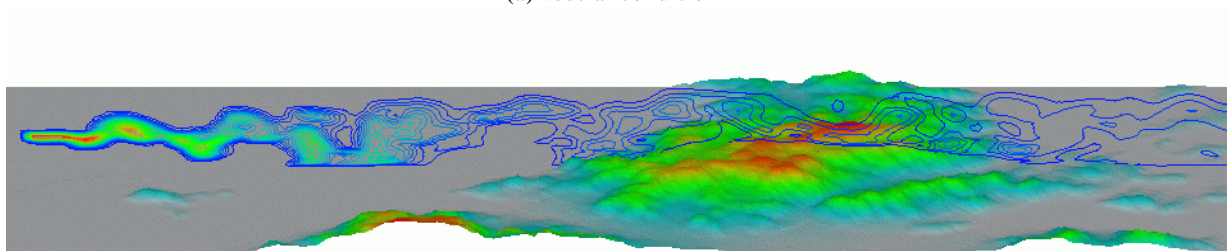
Fig.9 Comparison of the instantaneous flow field, t=80(s) , y=0 , smoke source height=0.97h
