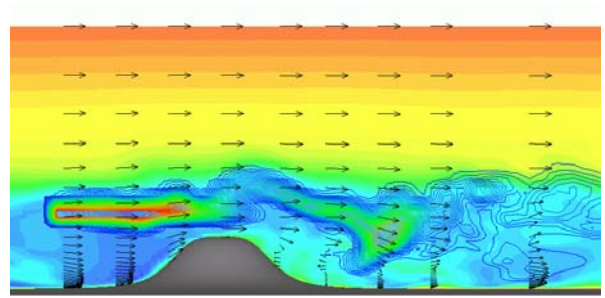
(c) Smoke source height=1.5h
