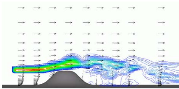
(a) Instantaneous flow field, t=70(s)
