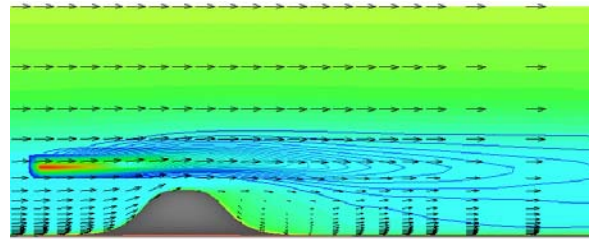
(b)Smoke source height=1.5h
