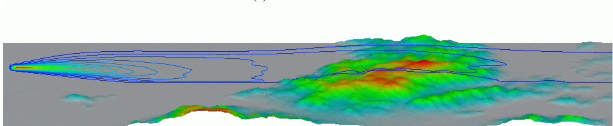
Fig.10 Comparison of the time-averaged flow field, t=60-80(s) , y=0 , smoke source height=0.97h
