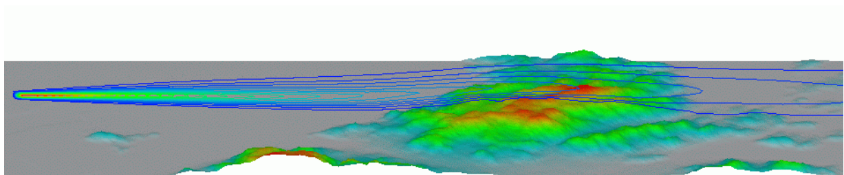
Fig.9 Comparison of the instantaneous flow field, t=80(s) , y=0 , smoke source height=0.97h
